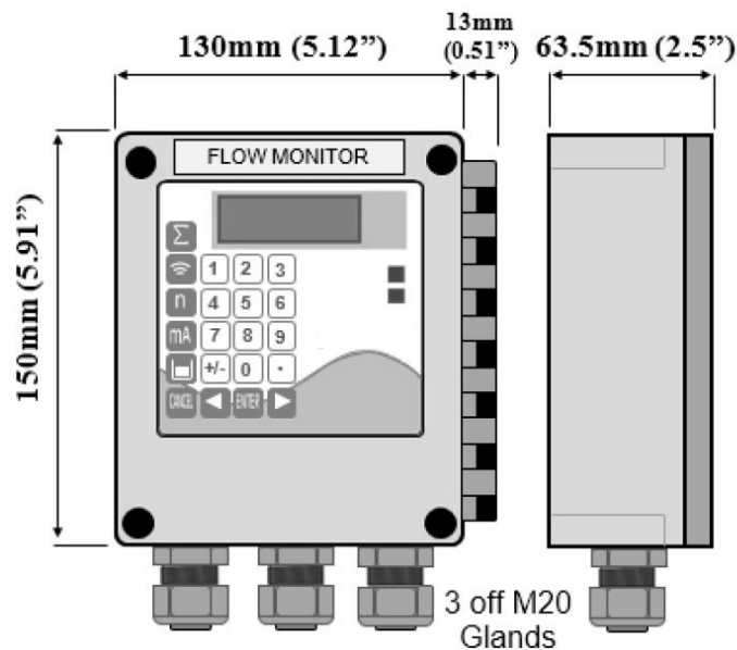
Flow Monitor Front and Side Drawing
